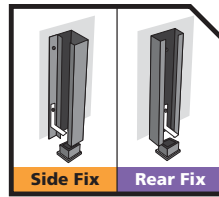
Install Screen Up channels
